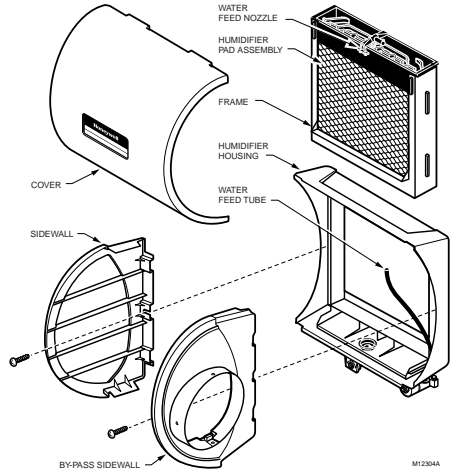
Fig. 3. Disassembling humidifier.
